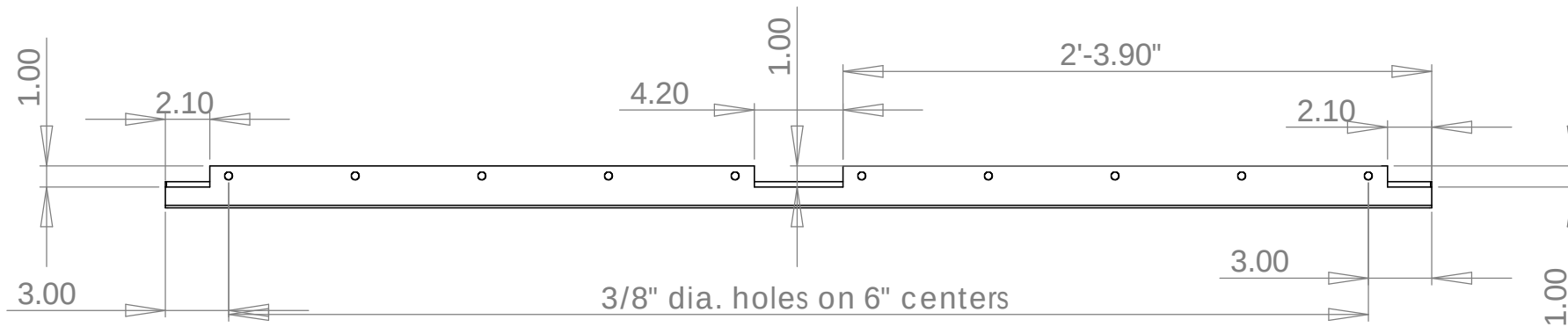
2" flange hole pattern
