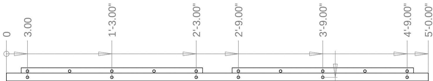
1-1/4" flange hole pattern
